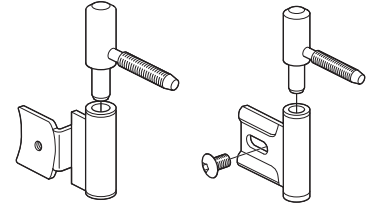
z-paumelle
